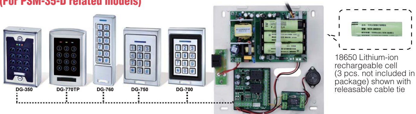
PSM-35-D Power Supply & Access Control Modules
